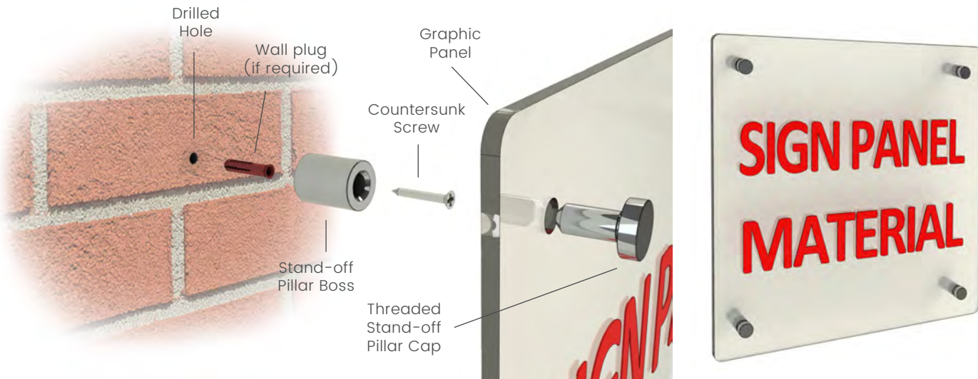
Screw Selection Guide
